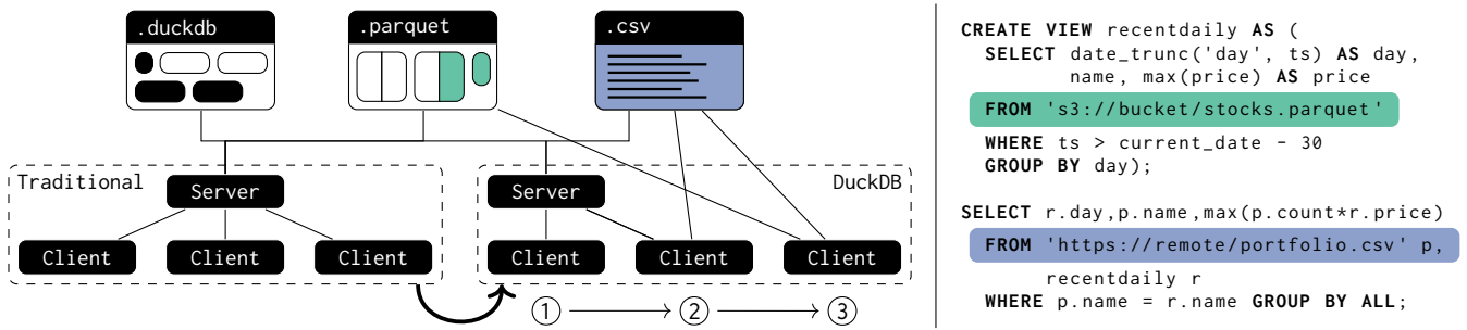
Figure 2: A SQL script that downloads stock data from AWS S3 stored in a Parquet file and joins it with a portfolio stored in a CSV file. The left side presents multiple ways to execute the script in a distributed setting. ① shows the traditional separation between client and server, ③ a fully local execution, ② a hybrid mode in between.
