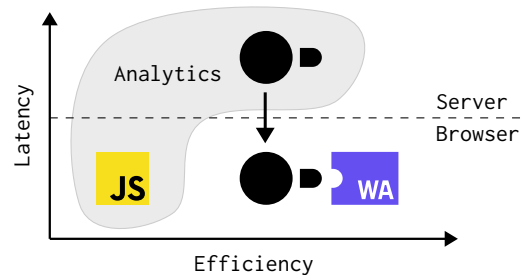
Figure 1: Browser-based analytics tools process data either locally with a low efficiency or on servers with a high latency. DuckDB-Wasm pushes the boundaries with fast analytical processing for the Web.
