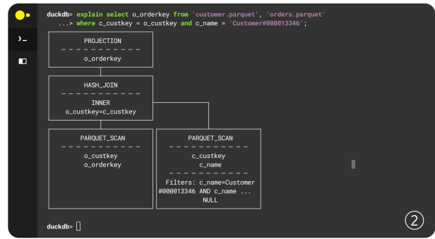
Figure 3: A shell that runs entirely in the browser and evaluates SQL queries using DuckDB-Wasm. The figure shows a query joining two parquet files with the relations orders and customer of the TPC-H benchmark at scale factor 0.1. ① lists the query results and page accesses, ② shows the query plan.
